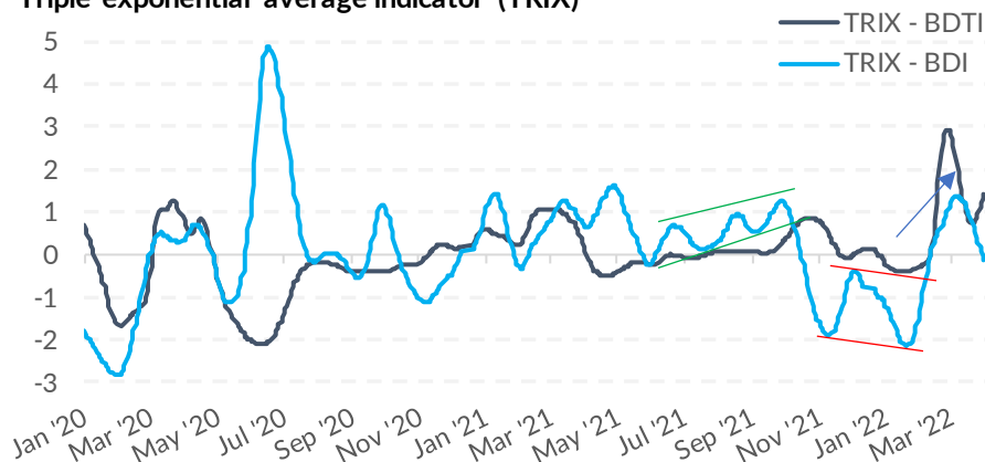
Triple exponential average indicator (TRIX)
